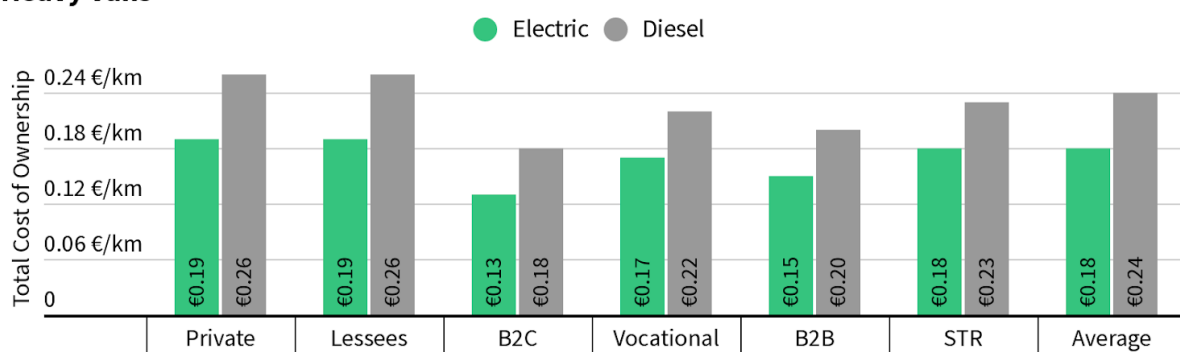
Figure 23: Average TCO of electric vans including subsidies and diesel vans in 2022 by user group
