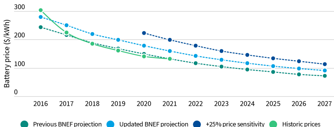
Figure 15: Battery prices as forecasted by BNEF, and higher prices used as part of the sensitivity analysis
